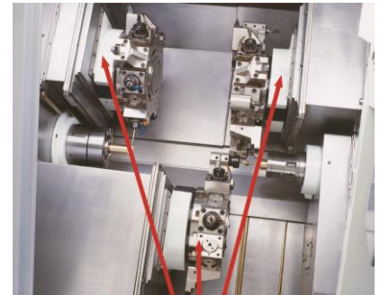
Three Y-Axis Turrets 288 Cutting Tool Capability
