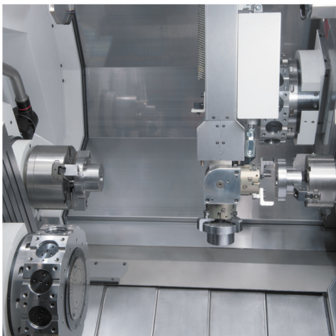
unload/load sub-spindle
